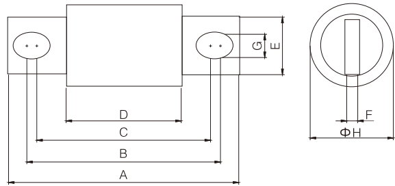
尺寸/Dimensions—mm
